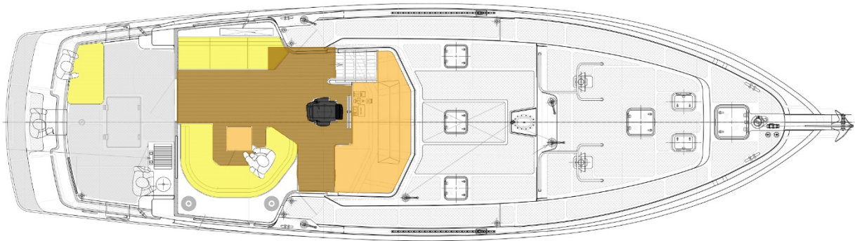
LAYOUT: Upper Level – Aft Deck and Saloon/Pilothouse:
